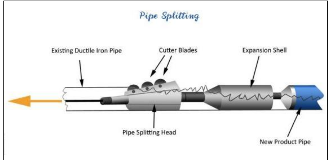
Pipe Splitting
