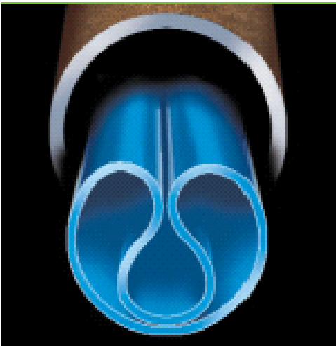
Shape of folded pipe during installation
